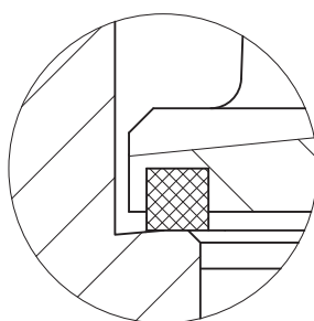
Weichdichtender Kegel Soft seated cone
